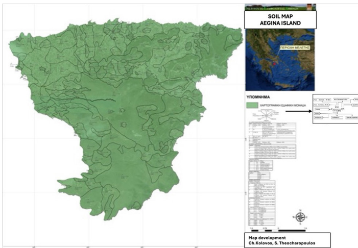
Figure 1. Soil map of Aegina Island in Greece (LIFE Agrostrat, 2017).
